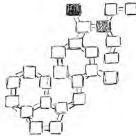
LSD
