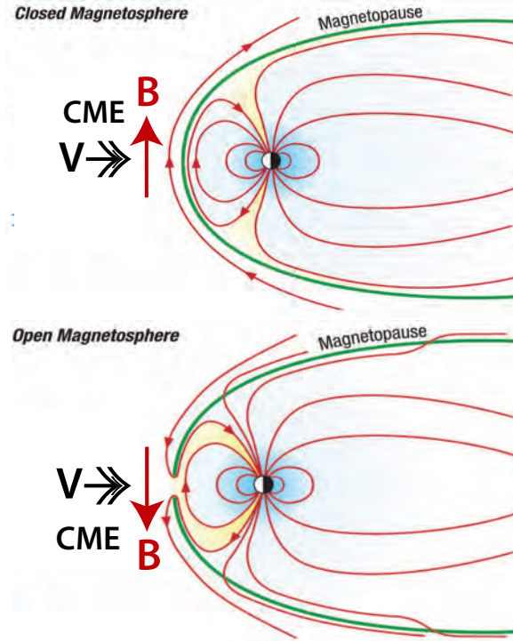
Figure 4: Schematic of CME impacting the magnetosphere, adapted from [17]. In the upper panel, the CME’s magnetic field vector is parallel to earth’s which repels it magnetically, although the impact compresses the magnetosphere’s bow wave. In the lower panel, the anti-parallel CME magnetic field connects with magnetosphere field lines in the bow wave, opening it to plasma in the CME.
