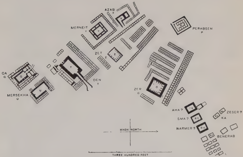
GENERAL PLAN OF TOMBS OF PREDYNASTIC AND FIRST DYNASTY PHARAOHS AT ABYDOS.
