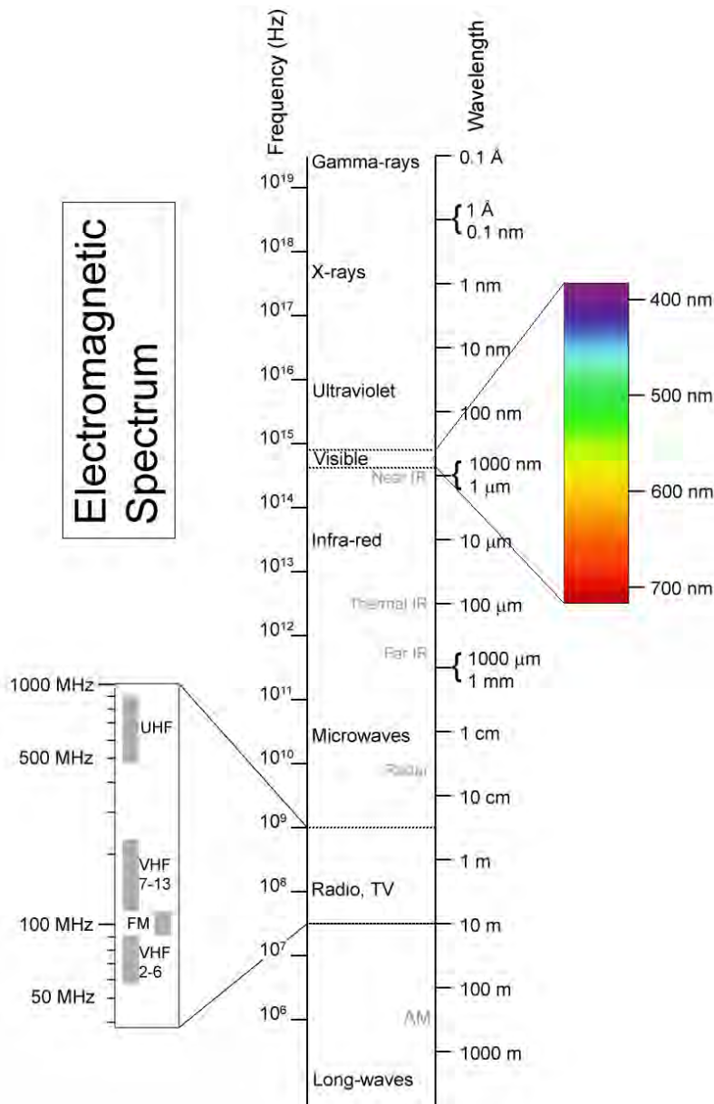
Diagram 1: Electromagnetic Spectrum
