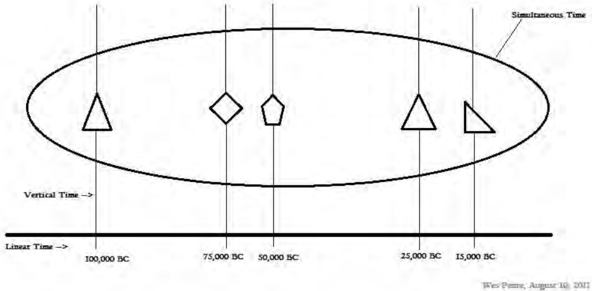
Diagram IC: Simultaneous Time (click on image to enlarge)
