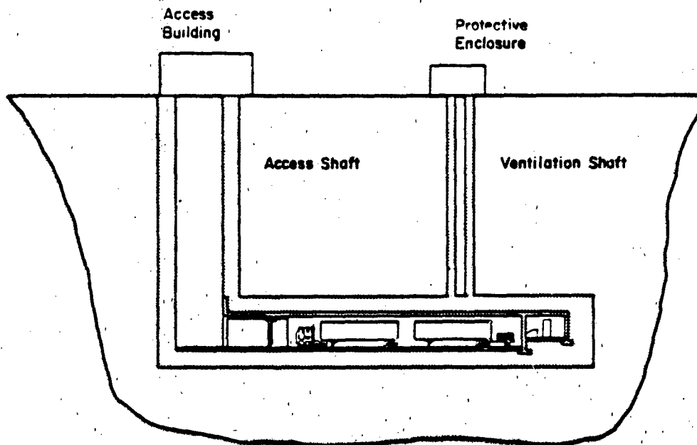
Figure 8. Deep shaft structures.
