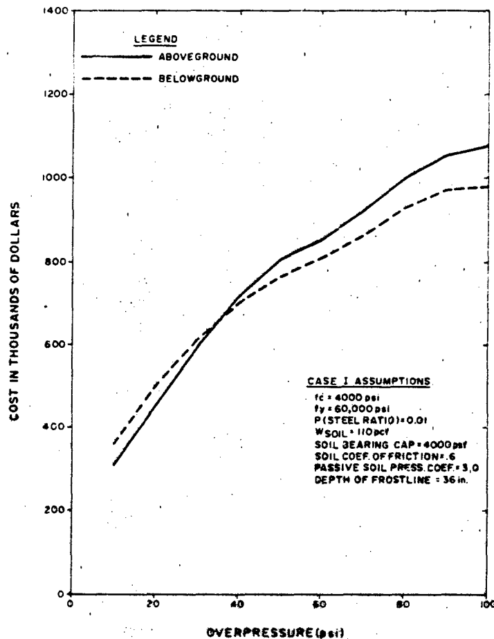
Figure 3. Cost vs. overpressure for example structures.
