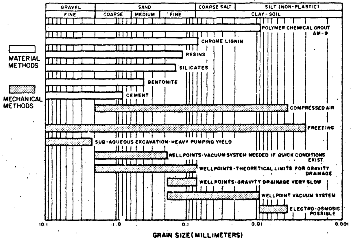
Figure 2. Comparison of methods for stabilizing and dewatering soil. (From Reference 22.)
